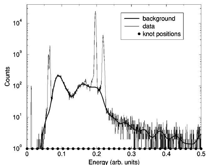
FIG. 1. A PIXE spectrum for a geological sample with the background estimate obtained in Ref. [1] using 35 evenly spaced spline knots. The oscillations in the estimated background above the energy of 0.25 seem unwarranted, given the large uncertainties in the measurements in this region.
