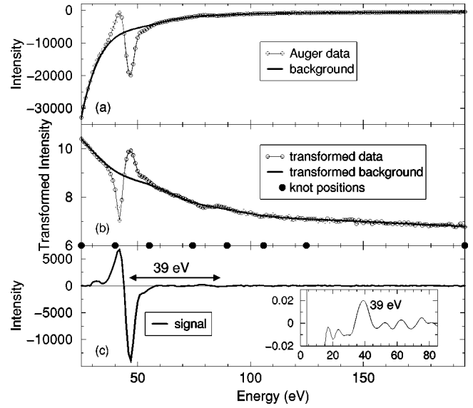
FIG. 6. (a) An MVV Auger spectrum for iron. The estimated background shown is that obtained for the transformed spectrum shown in (b). (b) A logarithmic transformation of the Auger spectrum shown in (a) reduces the curvature of the background, rendering it suitable for the general approach presented here. The estimated background is shown. (c) The signal determined by subtracting the estimated background from the original spectrum. The inset in (c) shows the autocorrelation of the signal vs energy difference. A significant secondary peak is seen at an energy offset of 39 eV.
