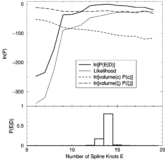
FIG. 3. The probability for the parameter E (the number of spline knots) given by Eq. (15), shown as the solid curve, with its various contributions. The maximum probability occurs at E=14 knots.
