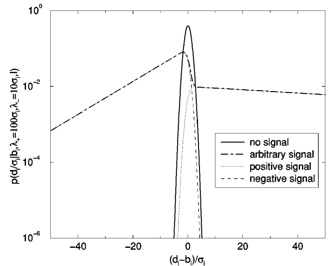
FIG. 2. The likelihood functions for the cases that there is no signal present, and for positive and negative signals of scales \lambda_- = 10\sigma and \lambda_+ = 100\sigma . The relative contribution of the latter to the mixture model (12) for the likelihood is weighted by 1-\beta , and the former by \beta .
