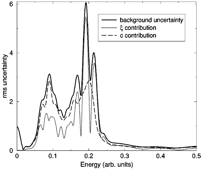
FIG. 5. The uncertainties in the background function displayed in Fig. 4. The separate contributions to the rms deviation of the background values are shown; from the uncertainties in the c and the variance arising from the knot positions \xi .
