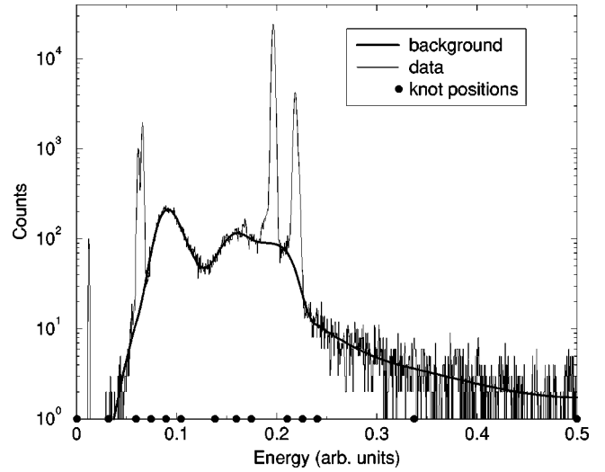
FIG. 4. The same PIXE spectrum as in Fig. 1, showing the most probable background estimate obtained using adaptive splines in which the optimal number of knots is found to be 14. In the energy region above 0.25, the estimated background is now smooth, indicating a lack of evidence in the data for the oscillations visible in Fig. 1.
